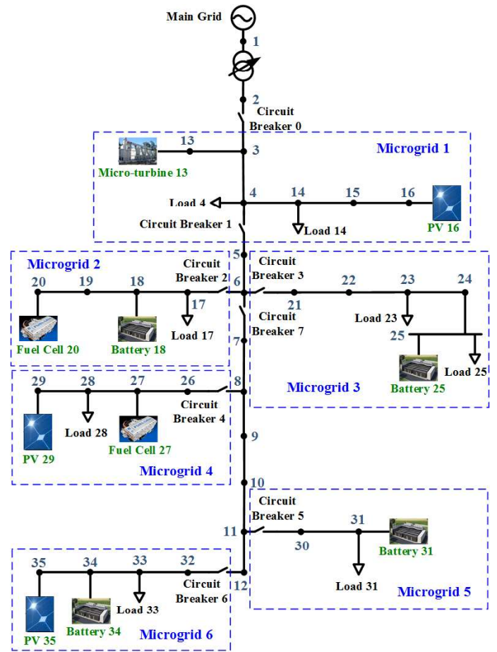
Fig. 4. A typical networked microgrids.
