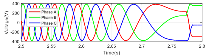
(a) Voltage response under cyberattack without SDASD
