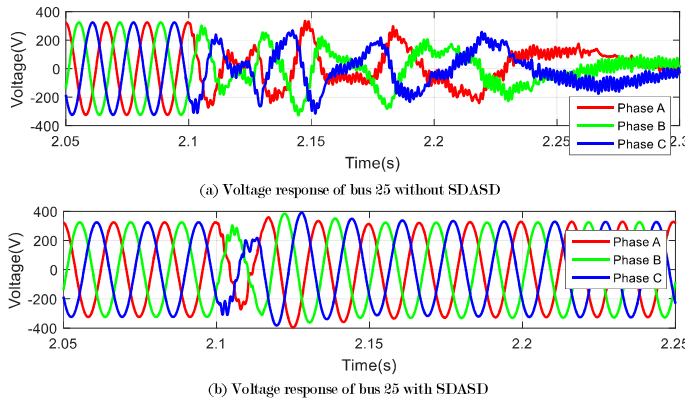
Fig. 19. Case 6: Voltage response of the bus 25 under simultaneous attacks.
