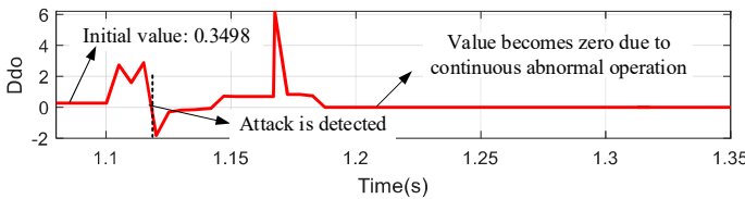
Fig. 15. Case 4: Detection results of D_{do} in Battery 18.
