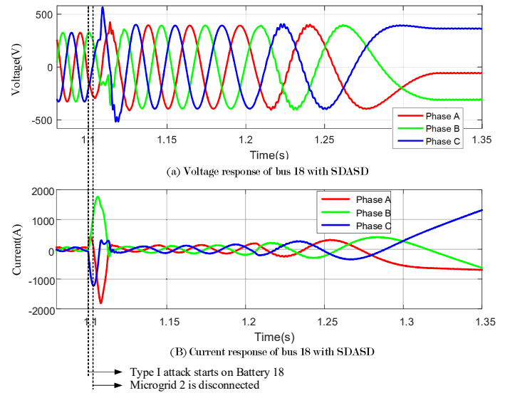
Fig. 13. Case 4: Voltage and current response of bus 18 with SDASD.
