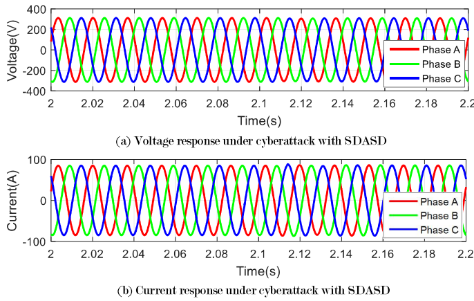
Fig. 10. Case 2: Voltage and current responses at bus 25.
