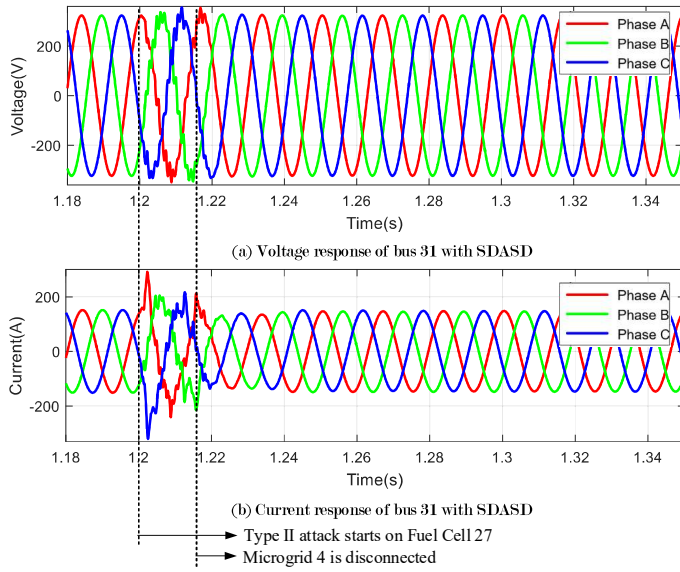
Fig. 18. Case 5: Voltage and current response of the bus 31 with SDASD.
