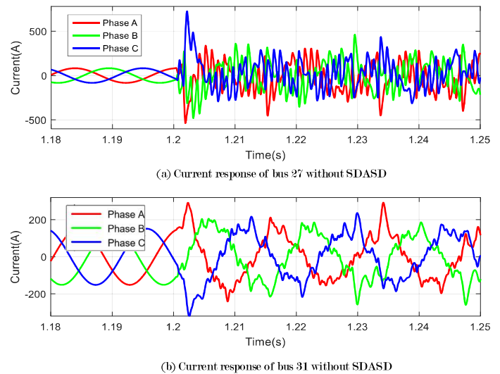
Fig. 16. Case 5: Current response of buses 27 and 31 without SDASD.
