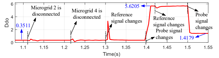
Fig. 21. Case 7: Detection results of D_{do} in Battery 34.
