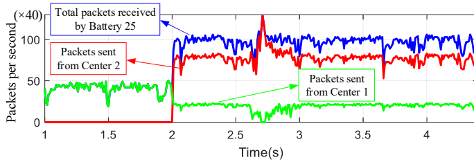
Fig. 6. Case1: Traffic monitoring (packet received by Battery 25).
