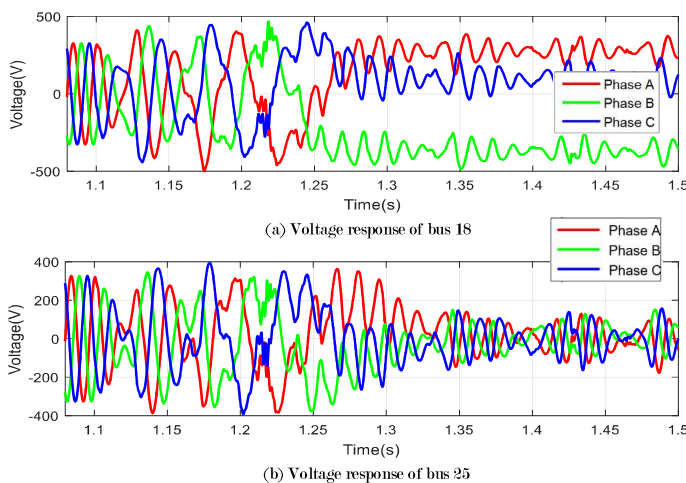
Fig. 12. Case 4: Voltage response of buses 18 and 25 without SDASD.
