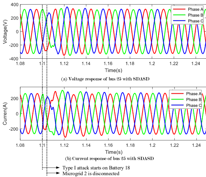
Fig. 14. Case 4: Voltage and current response of bus 25 with SDASD.
