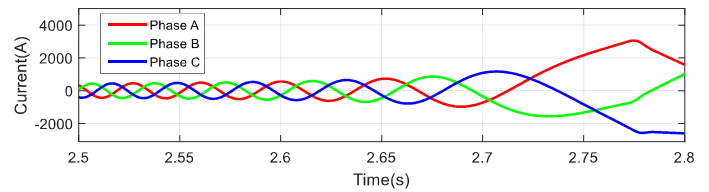
(b) Current response under cyberattack without SDASD
