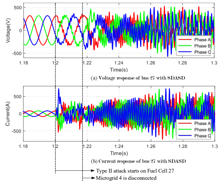
Fig. 17. Case 5: Voltage and current response of the bus 27 with SDASD.
