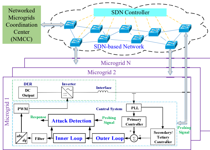
Fig. 1. SDASD architecture.
